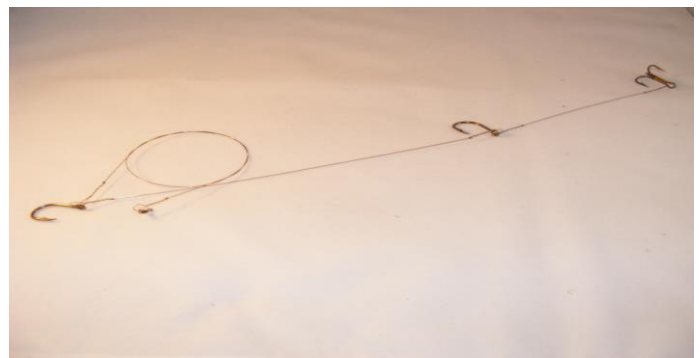
Double rig inline. Single strand #5 wire 2/0 single hooks, #4 Treble
