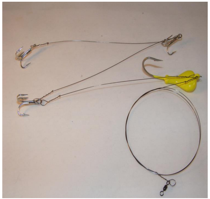
Ribbon fish rig Single Strand #5 wire, Blue Water Candy 1/2oz chartreuse jig head, #4 silver treble hooks
