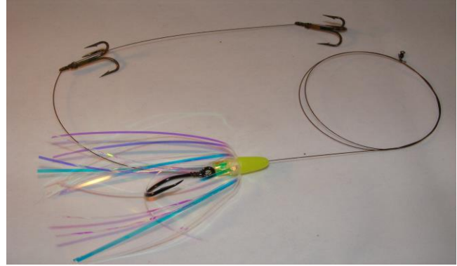
1x7 wire 60lb, 4/0 single hook, (2) #2 trebles. Blue Water Candy Privat skirt
